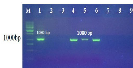
Fig4: The optimized PCR test for detects blaTEM gene in Clinical Samples
