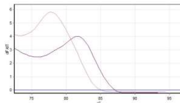
Figure 2. Melting curve of EGFR and FGFR4 genes in lung cancer cell line. The EGFR melting curve is at 81.5^{\circ}\text{C} and the FGFR4 melting curve is at 77.8^{\circ}\text{C} . The vertical axis indicates the fluorescent derivative to the time derivative and the horizontal axis represents the temperature at ^{\circ}\text{C} . The single-peak in the diagrams indicates the absence of a primer dimer and a non-specific bond.
