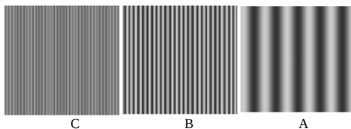
Figure1. Types of visual stimuli used in the study at various spatial frequencies: low spatial frequency (a), middle spatial frequency (b) and high spatial frequency (c).
