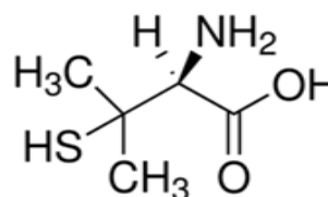
Figure 2. D-penicillamine (DPA)
