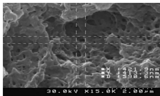
Figure 3. Porous morphology of CH-β-GP-HEC hydrogels after water removal by electron microscopy
